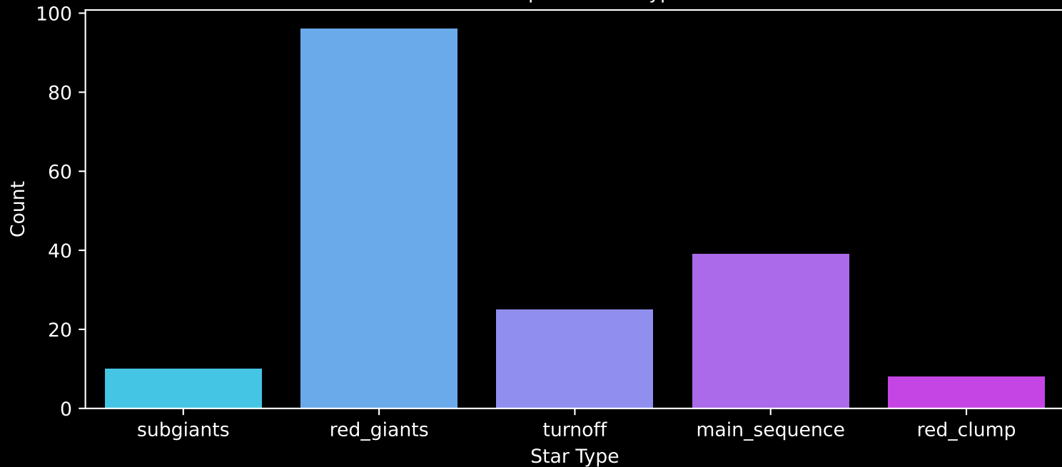
APOGEE DR17 Field: [277-35-O] Count plot of Star Type
