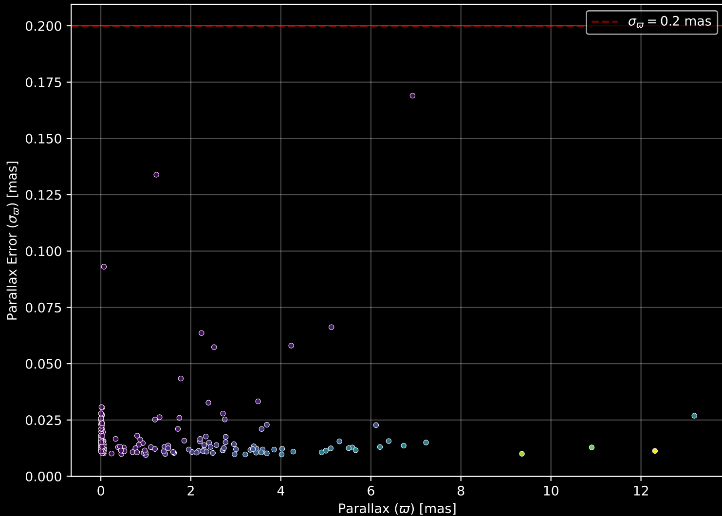
APOGEE DR17 Field: [277-35-O] Parallax Quality (n= 178)
