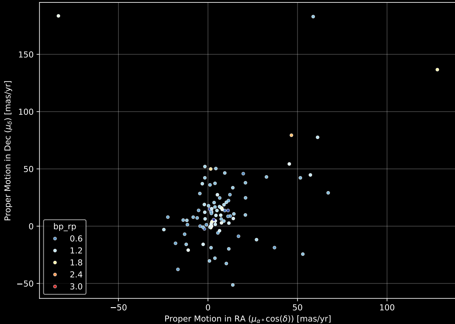
APOGEE DR17 Field: [277-35-O] Proper Motion Diagram (n= 178)
