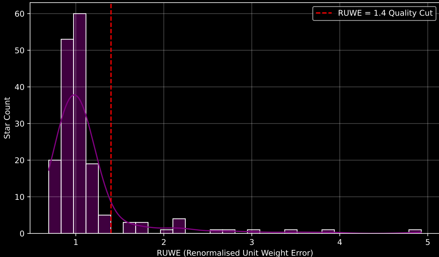
GAPOGEE DR17 Field [277-35-O] RUWE Distribution (n= 174)
