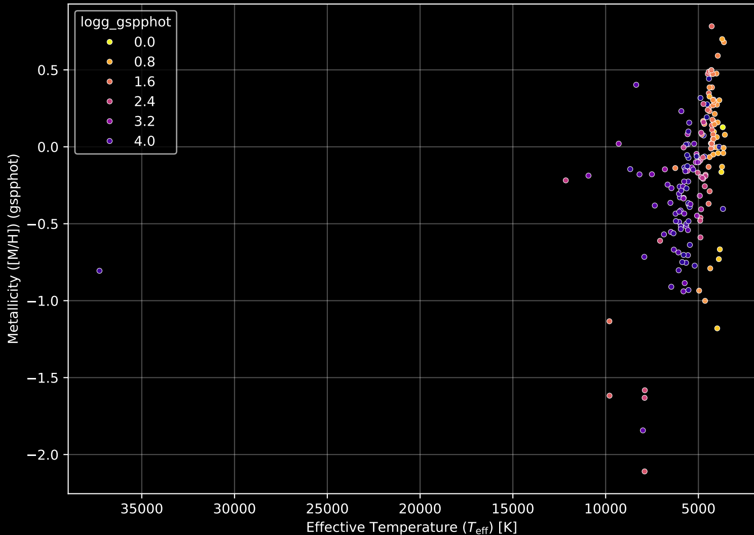
APOGEE DR17 Field: [277-35-O] Stellar Population Parameters (n= 178)
