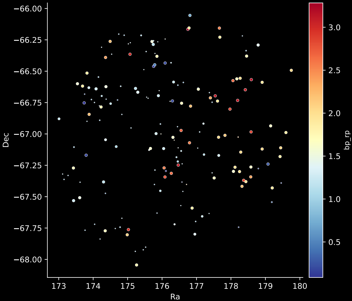
APOGEE DR17 Field: [277-35-O] Stars: 178
