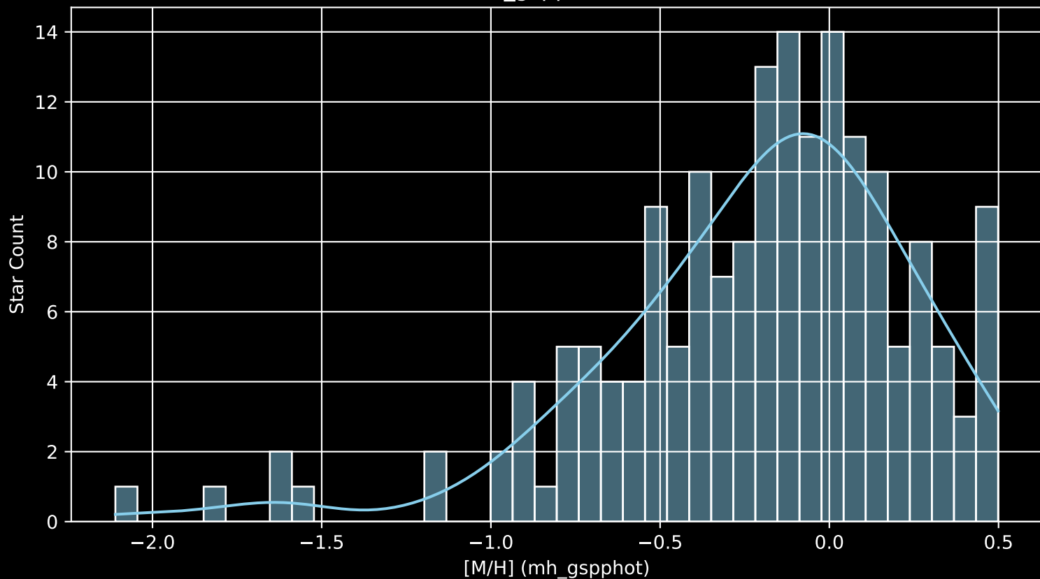
APOGEE DR17 Field: [277-35-O [M/H] (mh_gspphot) (n= 174)
